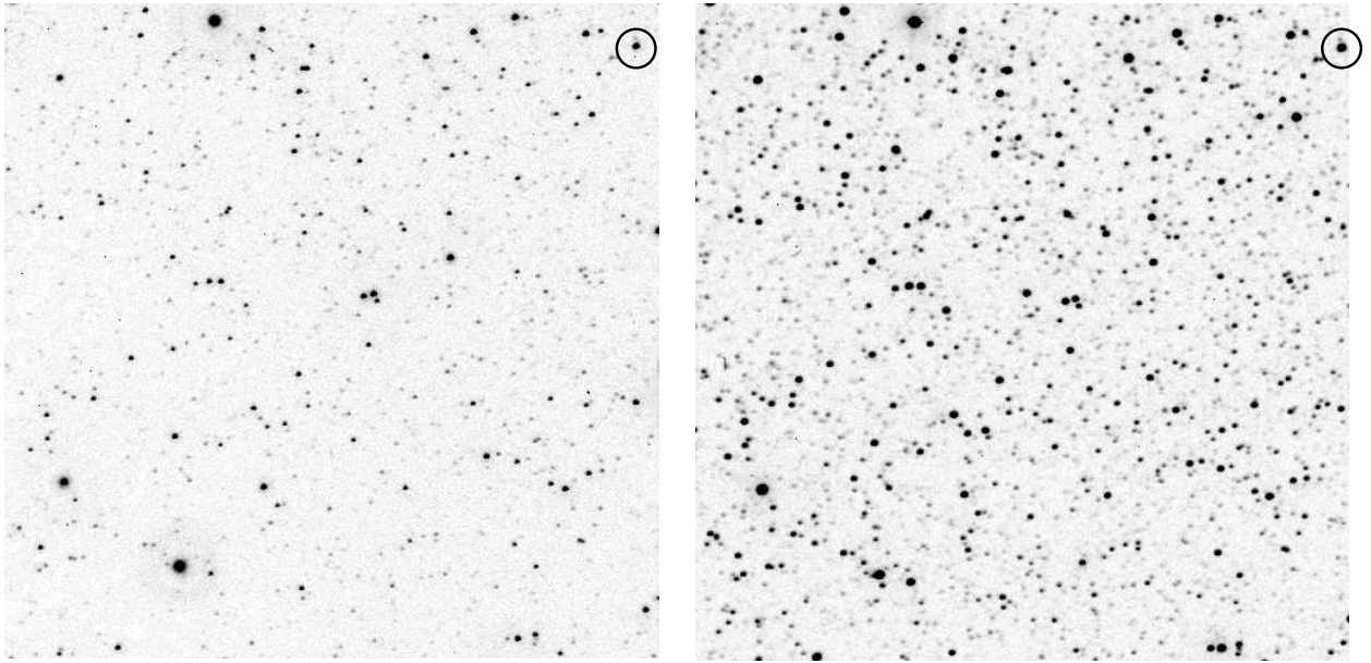
Fig. 1.— The central portion of a Mark IV image pair, a 1^\circ \times 1^\circ area centered at RA=20:16:14.2, Dec=+16:16:18, about 10 degrees from the galactic plane. V -band is on the left, I C -band on the right. North is up, East to the left. The circled star is R Sge.
