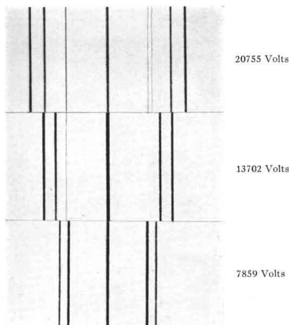
FIG. 9. Spectrograms obtained for several applied voltages.
