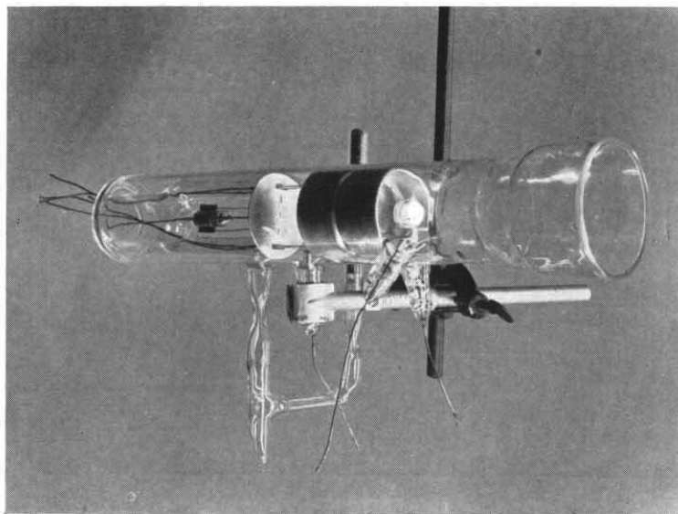
Fig. 3. Side view of canal-ray tube.
