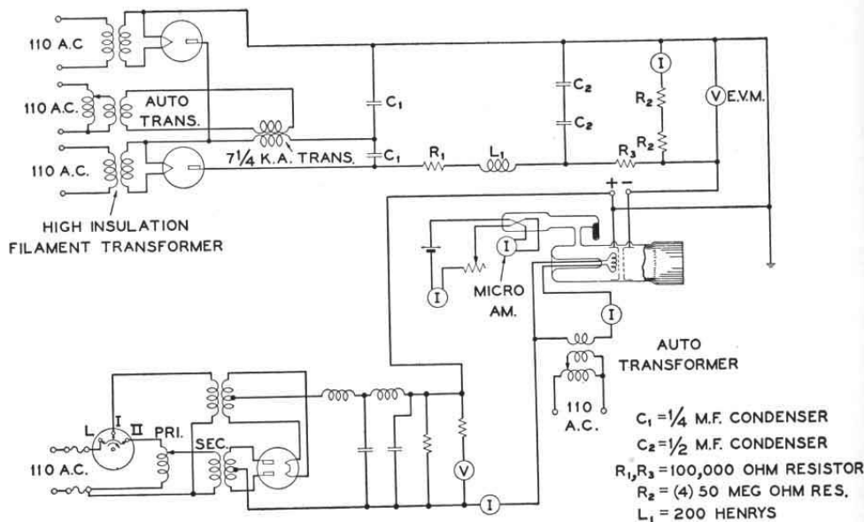
FIG. 5. Electrical circuits used with canal-ray tube.
