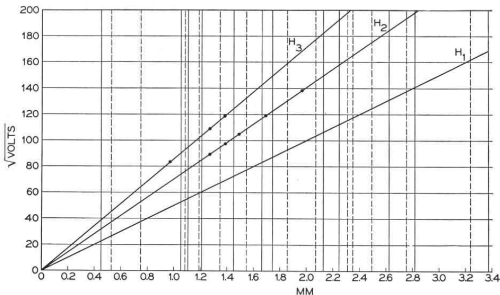
FIG. 12. Chief molecular spectrum lines of hydrogen in the neighborhood of H\beta . Lines to blue side shown full, to red side, dashed.
