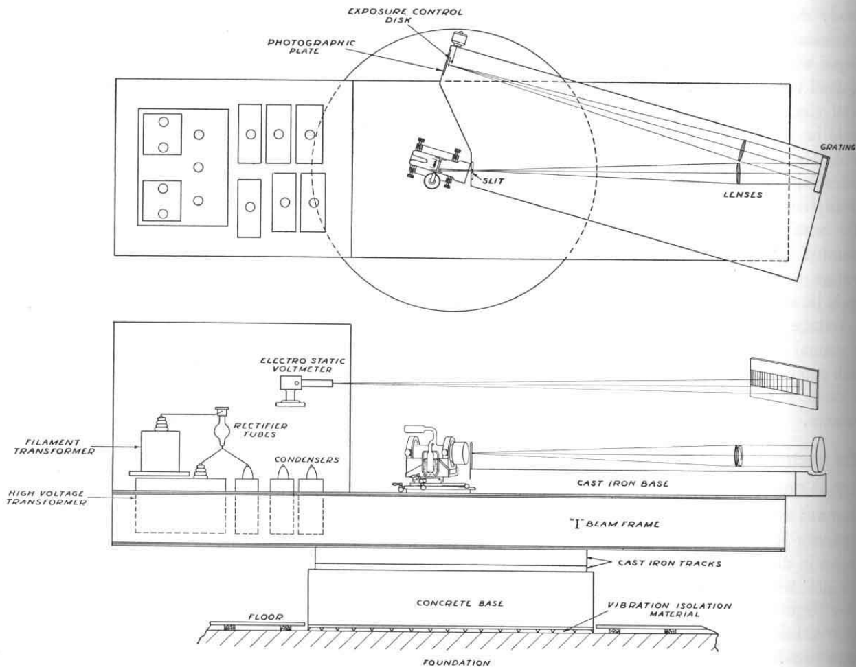
FIG. 6. Plan of apparatus.
