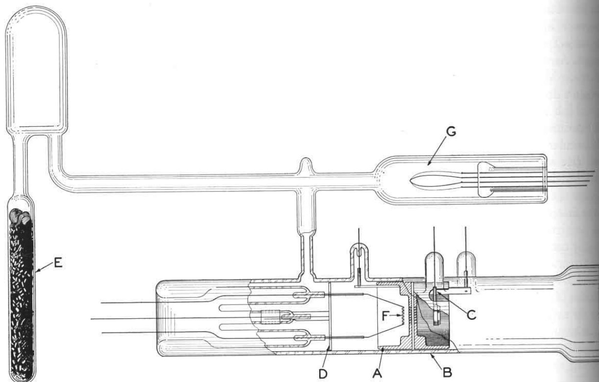
FIG. 2. Diagrammatic representation of canal-ray tube.
